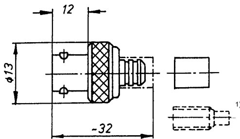
1) Crimp Sleeve adapted to the Cable Sheath
