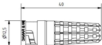
Cable Plug with Rotary Sleeve
